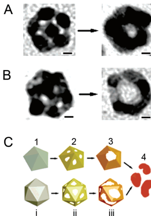
Figure 4. Morphological evolution for Ag MTPs with (A) decahedral and (B) icosahedral structure during the galvanic replacement reaction. Holes on {111} facets of the particle were clearly resolved. As the reaction proceeded, these holes eventually disappeared. Instead, a big void was formed in the middle of the particle. (C) Mechanisms proposed to account for the formation of hollow structures from oleylamine-capped Ag MTPs. When HAuCl 4 in CHCl 3 is injected to the Ag MTPs, pitting starts from the surfaces of the nanoparticles to form pinholes, which make the particles appear like nanocages (step 2). As the reaction proceeds, some ridges break due to consumption of the Ag, and some grow through the deposition of Au and Oswald ripening. Pinholes combine and form a big opening on the particles; the shape of the hollow particles evolves from nanocage into nanoring (step 3). Adding more HAuCl 4 after this stage would result in the collapse of the hollow particles and formation of small fragments (step 4). As the ratio of HAuCl 4 to Ag increased from step (1) to step (4), the compositional change from pure Ag to Ag–Au alloys is illustrated by different colors. The scale bars for (A) and (B) are 2 nm.
