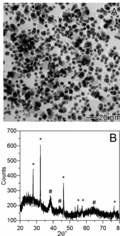
Figure 6. Galvanic replacement reaction between HAuCl 4 and oleylamine-capped Ag MTPs without adding extra oleylamine: (A) TEM image showing a mix of few hollow particles and a lot of irregularly shaped large particles. (B) XRD of the sample revealing the coexistence of peaks for both Ag-Au alloy (#) and AgCl (*).
