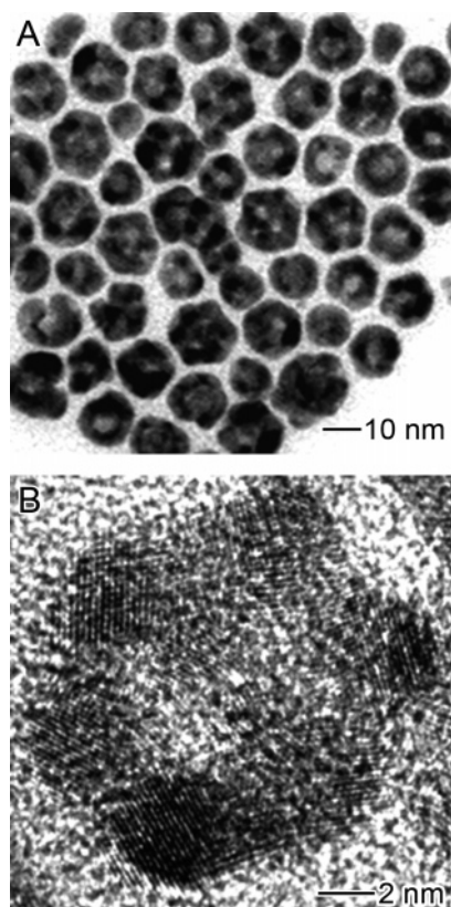
Figure 3. (A) Nanocages derived from 14.0-nm Ag nanoparticles by reacting with 1.2 mL of 0.5 mM HAuCl 4 in CHCl 3 . The average size of the hollow particles increased to 15.1 ± 2.1 nm. A majority of the particles exhibit the cage-like morphology. (B) HRTEM of a nanocage. Note that the lattice fringes are missing in some regions, corresponding to holes on the surface.
